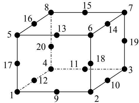
*HEXAHEDRONS_20
