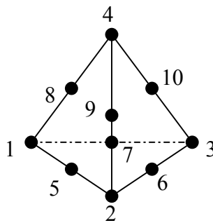
*TETRAHEDRONS_10
