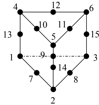
*PENTAHEDRONS_15
